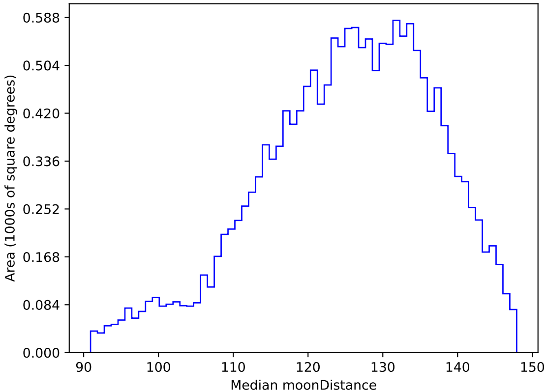
baseline_v3.3_10yrs WFD u band: Median moonDistance
