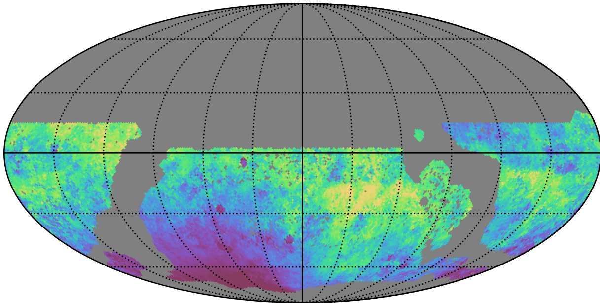
baseline_v3.3_10yrs WFD r band: Median moonDistance
