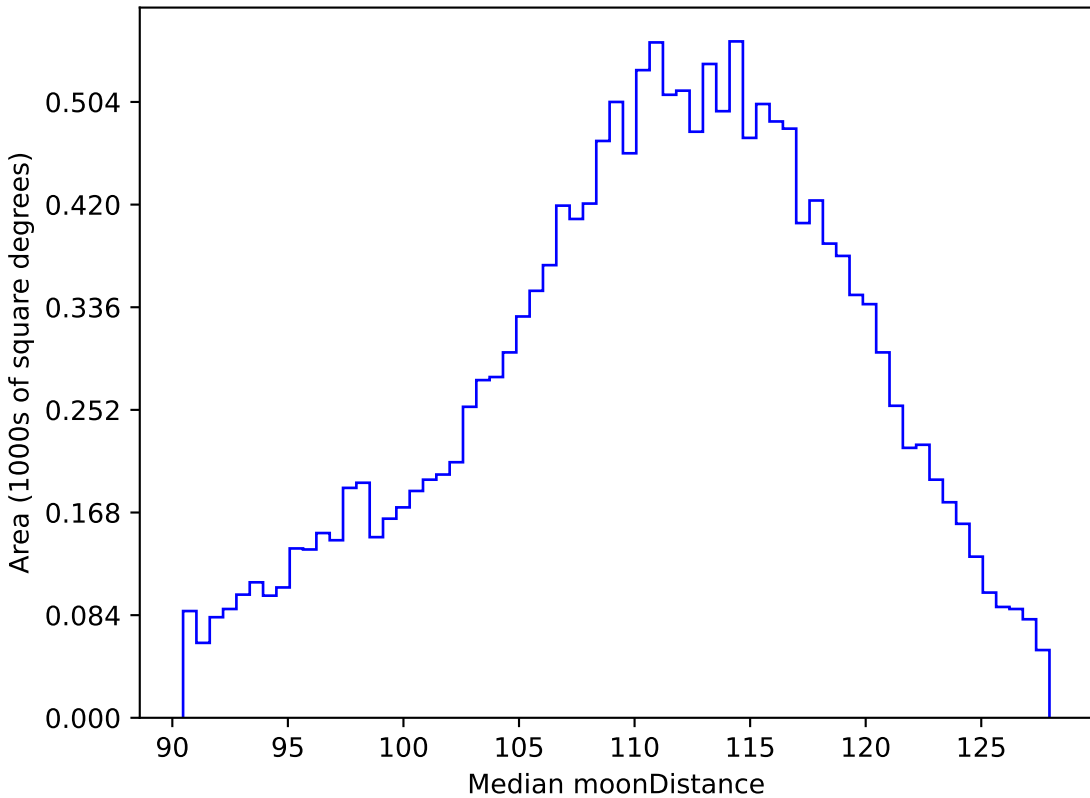
baseline_v3.3_10yrs WFD r band: Median moonDistance
