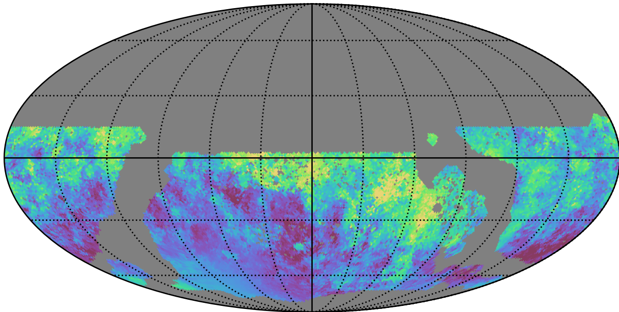
baseline_v3.3_10yrs WFD i band: Median moonDistance
