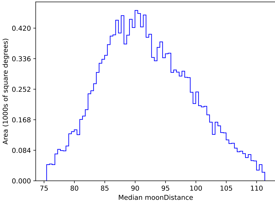
baseline_v3.3_10yrs WFD i band: Median moonDistance
