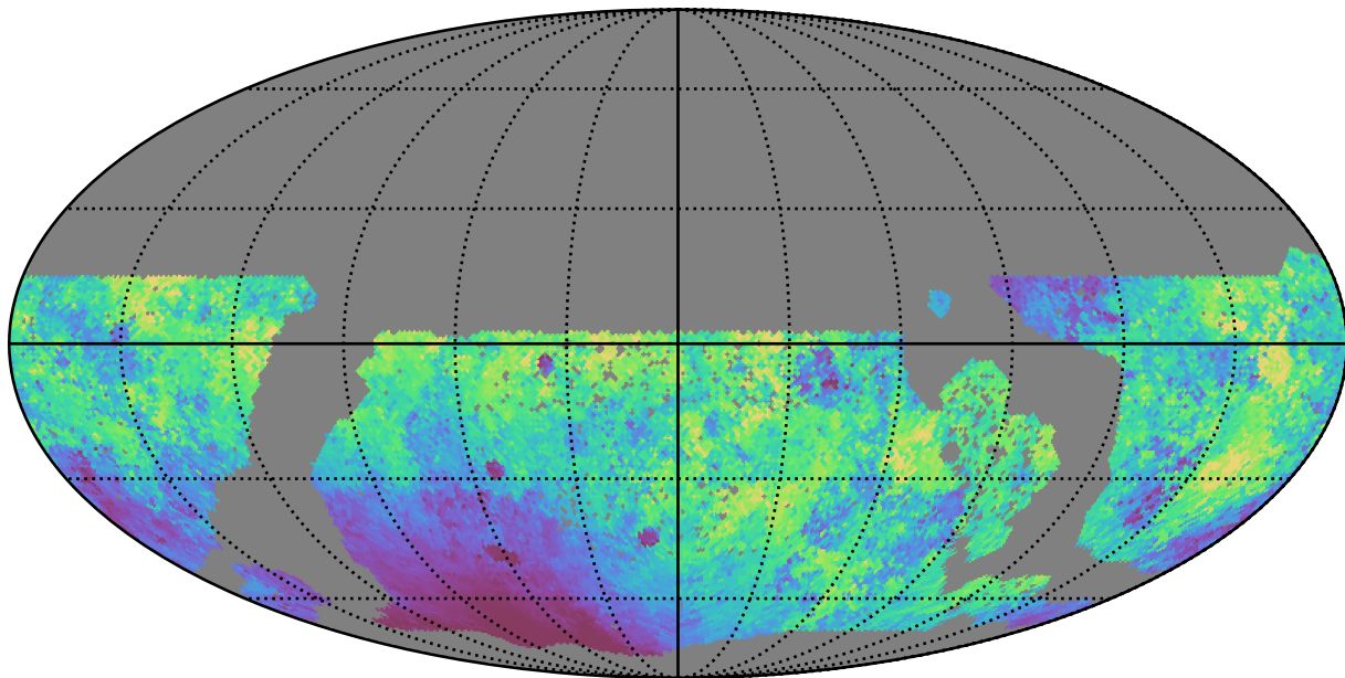
baseline_v3.3_10yrs WFD g band: Median moonDistance
