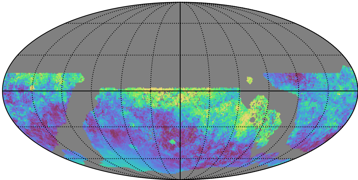
baseline_v3.3_10yrs WFD all bands: Median moonDistance
