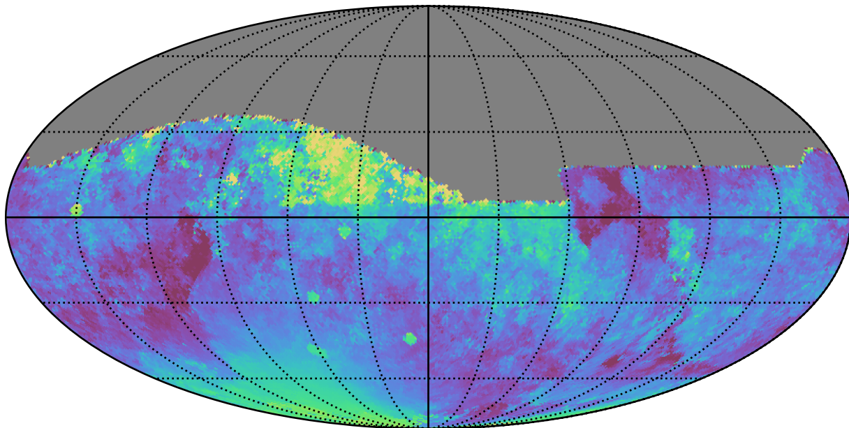
baseline_v3.3_10yrs All sky z band: Median moonDistance
