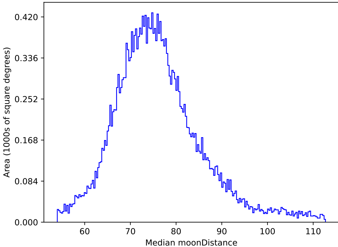
baseline_v3.3_10yrs All sky z band: Median moonDistance
