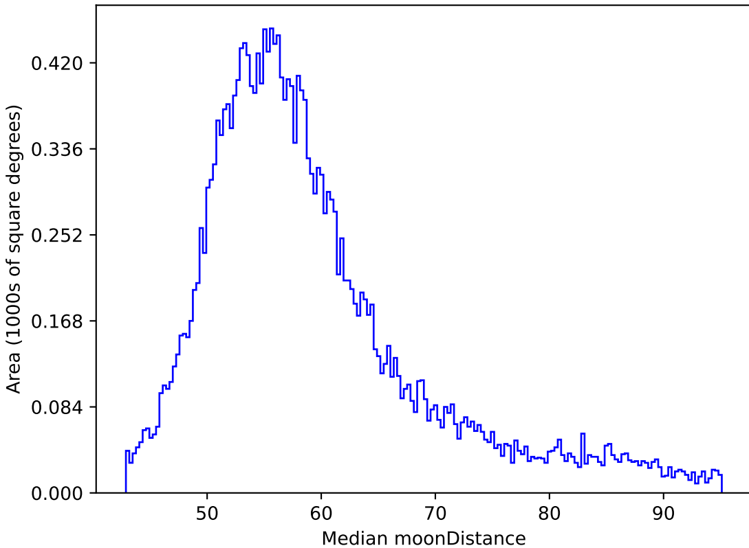
baseline_v3.3_10yrs All sky y band: Median moonDistance
