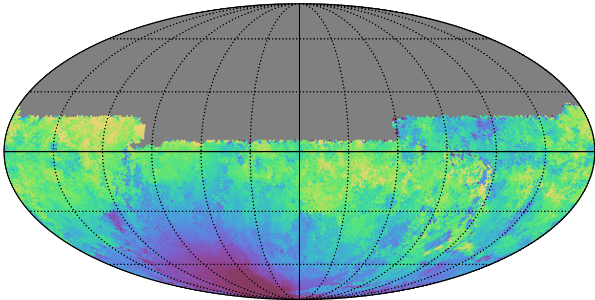
baseline_v3.3_10yrs All sky u band: Median moonDistance
