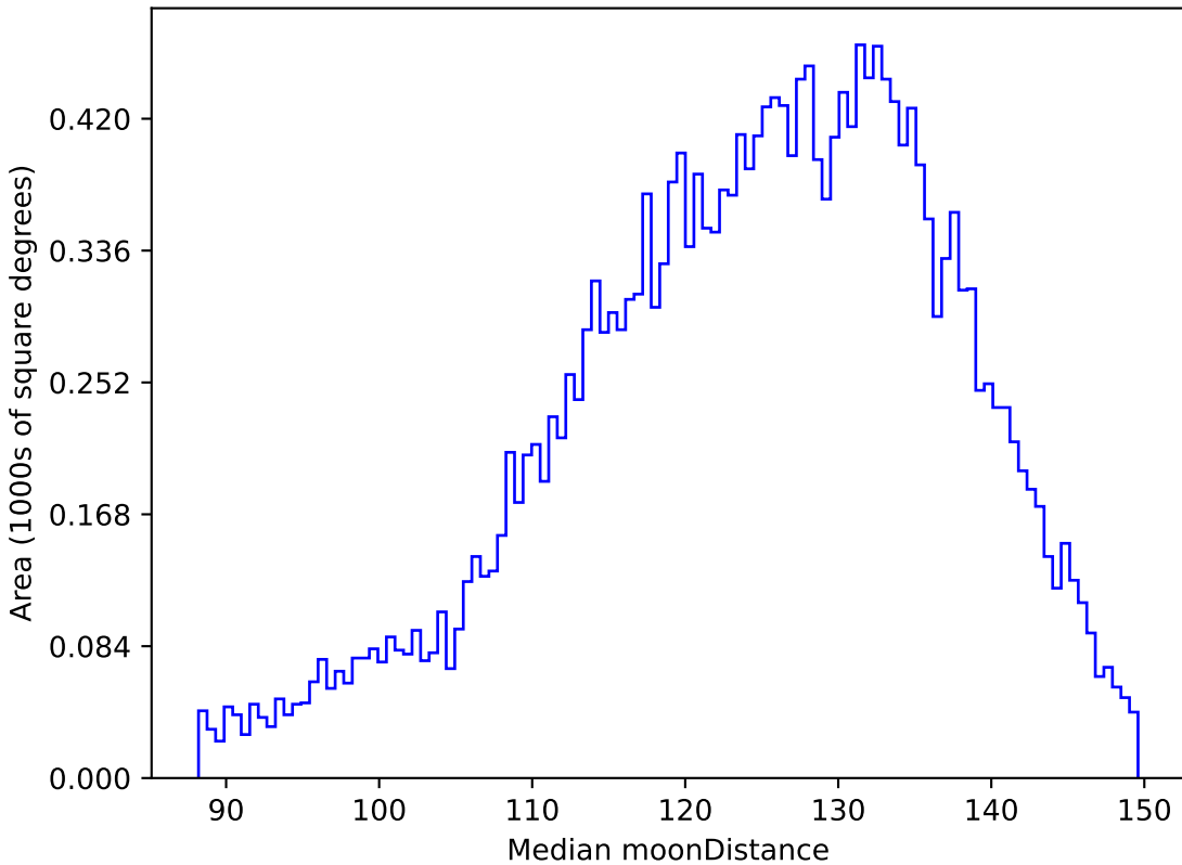
baseline_v3.3_10yrs All sky u band: Median moonDistance
