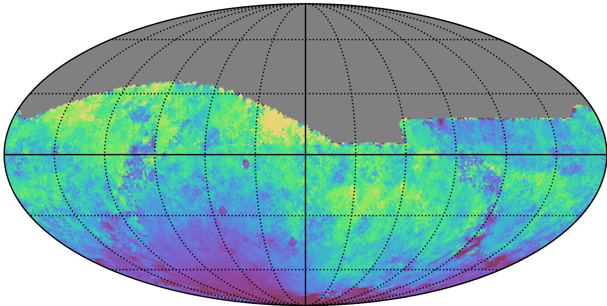
baseline_v3.3_10yrs All sky r band: Median moonDistance
