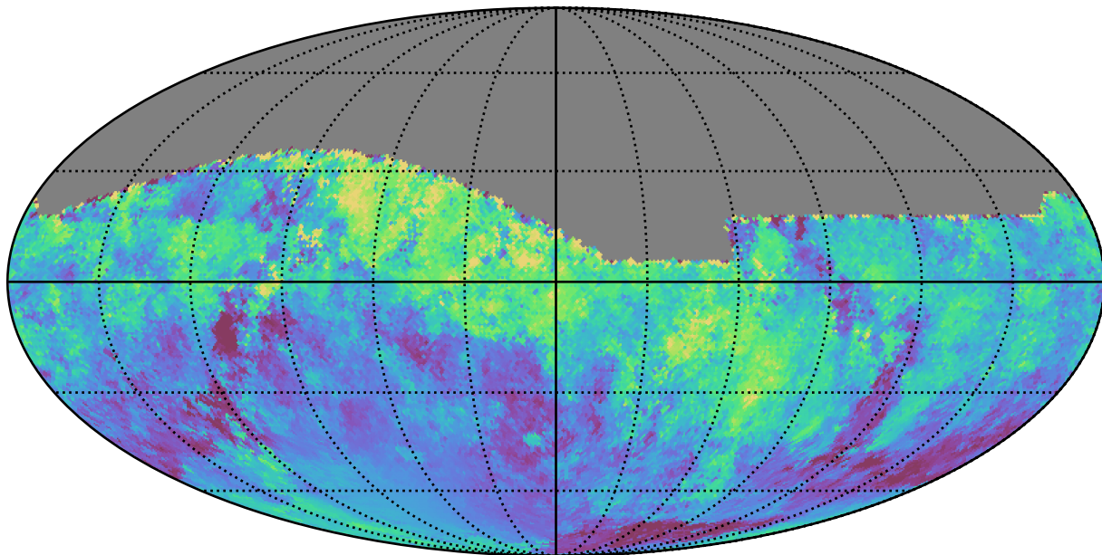
baseline_v3.3_10yrs All sky i band: Median moonDistance
