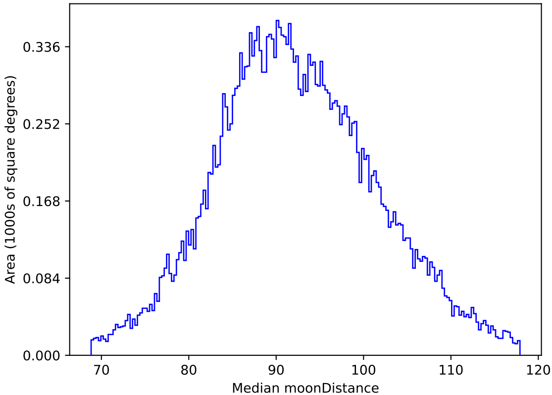
baseline_v3.3_10yrs All sky i band: Median moonDistance
