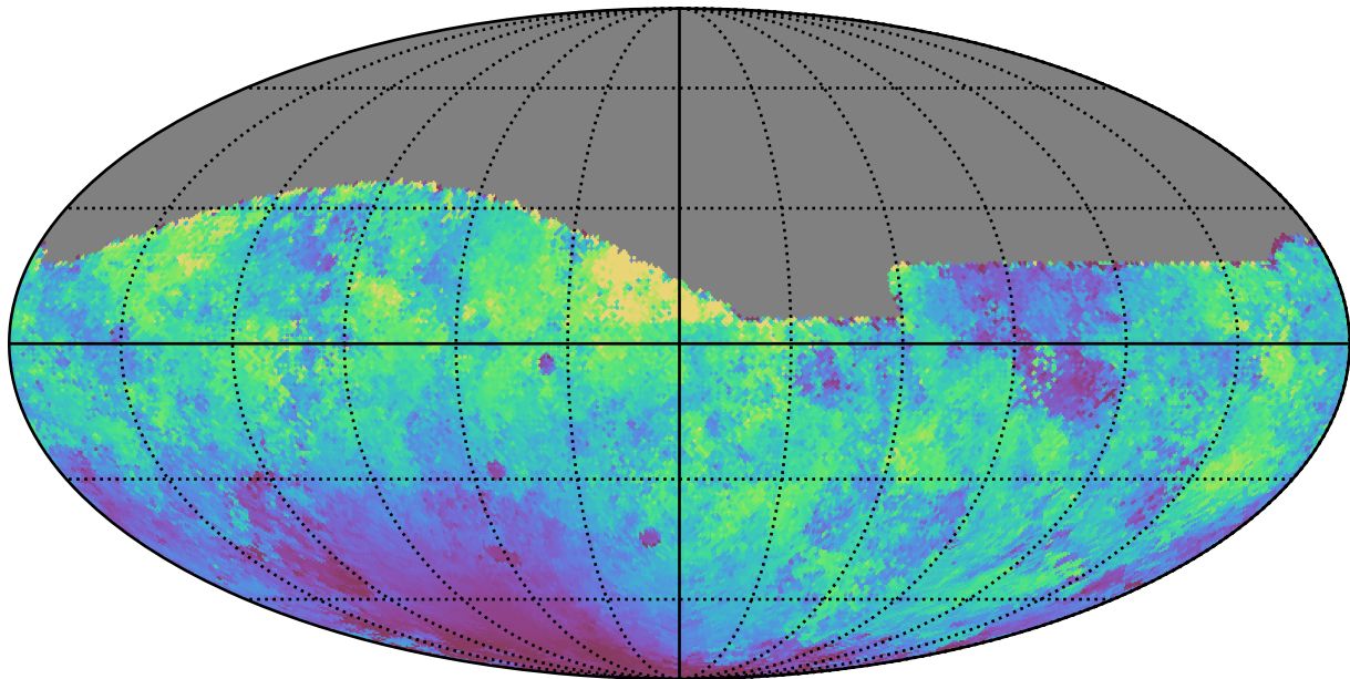
baseline_v3.3_10yrs All sky g band: Median moonDistance
