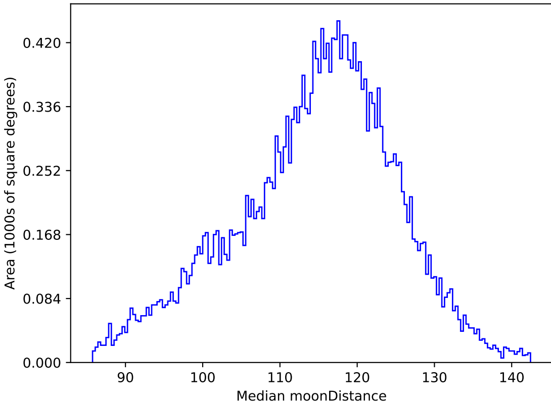
baseline_v3.3_10yrs All sky g band: Median moonDistance
