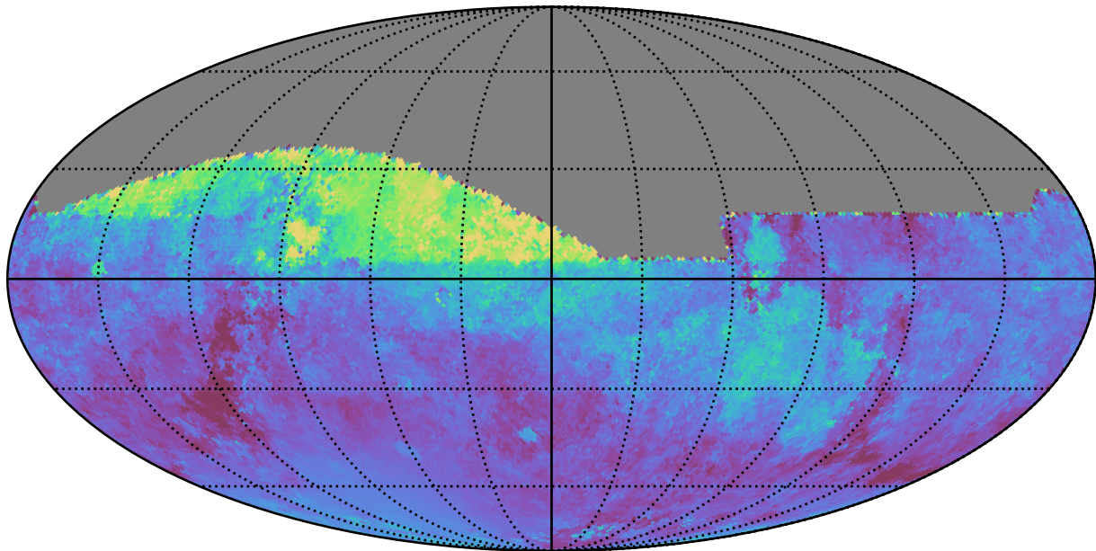
baseline_v3.3_10yrs All sky all bands: Median moonDistance
