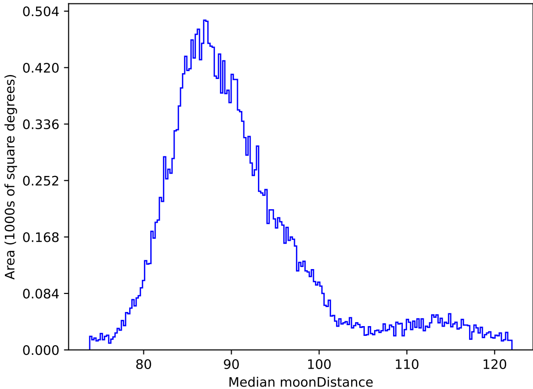
baseline_v3.3_10yrs All sky all bands: Median moonDistance
