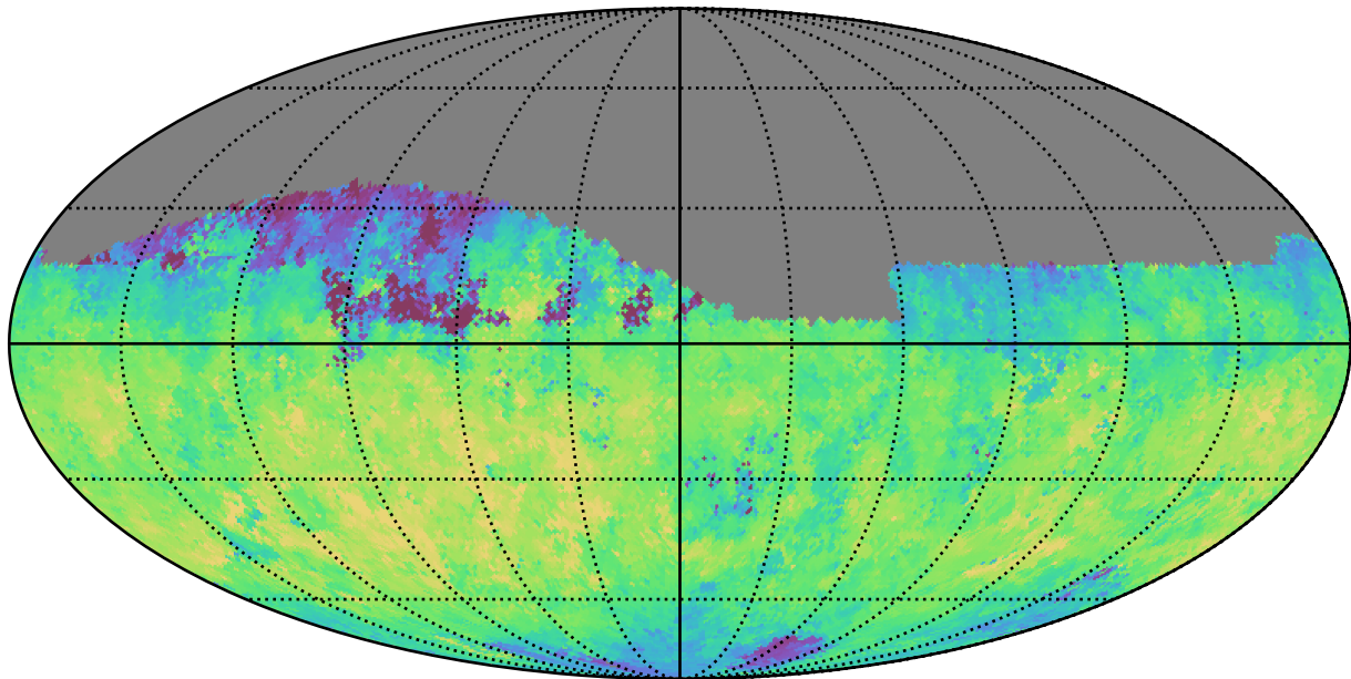
baseline_v3.3_10yrs Yr 1 z band: Median fiveSigmaDepth
