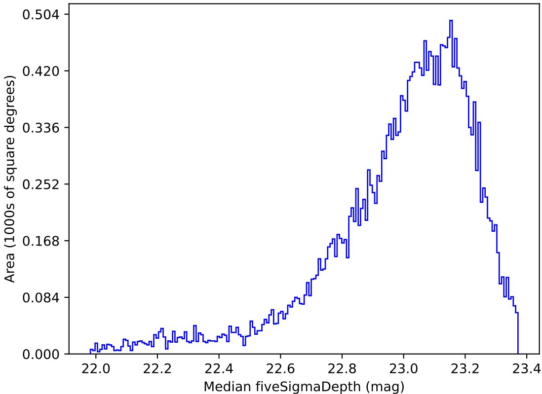
baseline_v3.3_10yrs Yr 1 z band: Median fiveSigmaDepth
