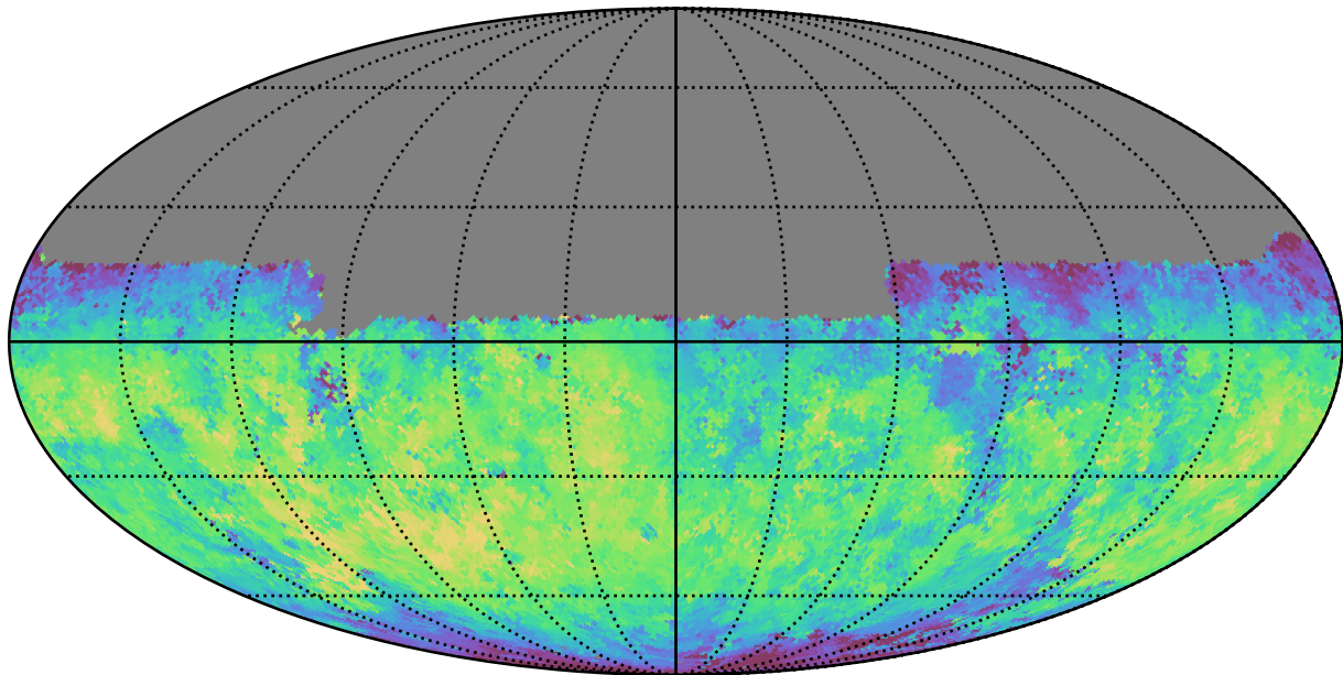
baseline_v3.3_10yrs Yr 1 y band: Median fiveSigmaDepth
