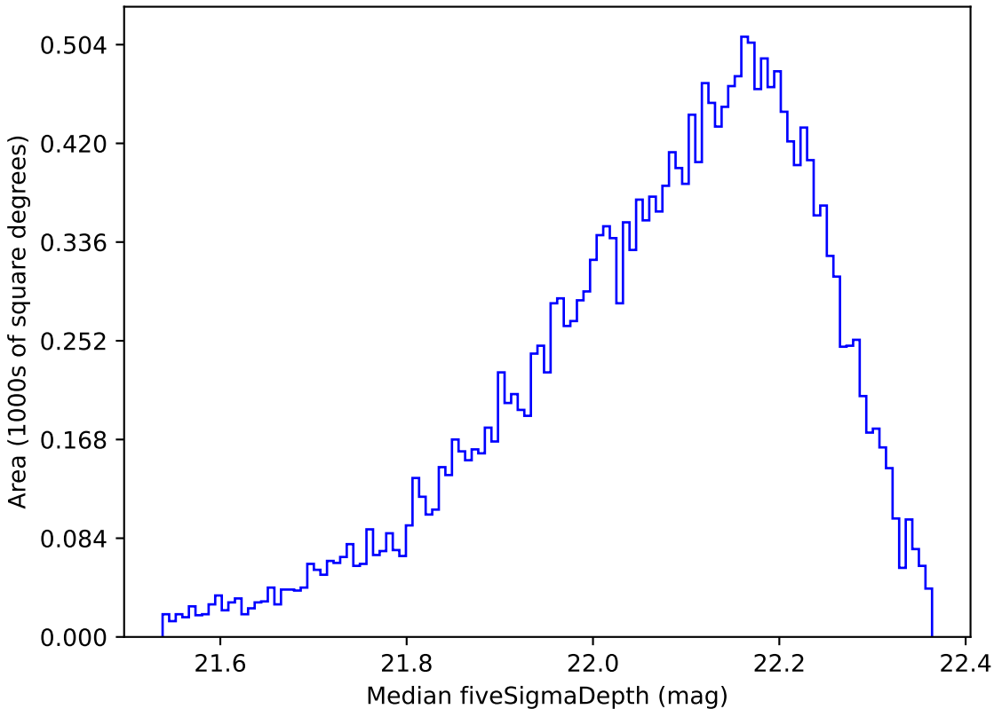
baseline_v3.3_10yrs Yr 1 y band: Median fiveSigmaDepth
