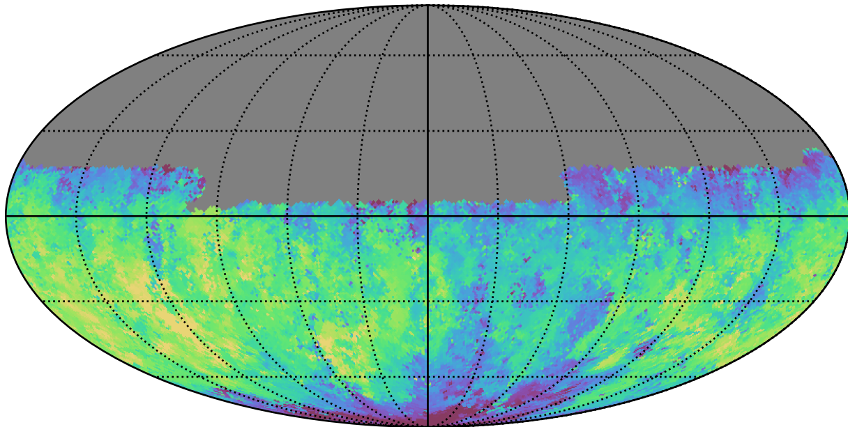
baseline_v3.3_10yrs Yr 1 u band: Median fiveSigmaDepth
