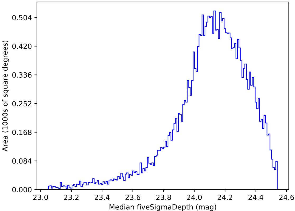
baseline_v3.3_10yrs Yr 1 r band: Median fiveSigmaDepth
