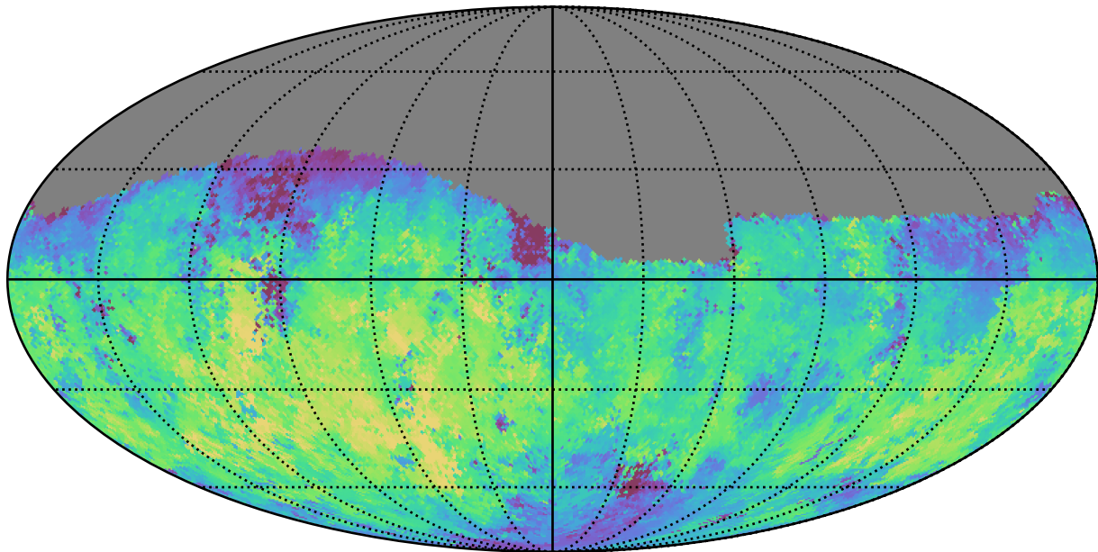
baseline_v3.3_10yrs Yr 1 g band: Median fiveSigmaDepth
