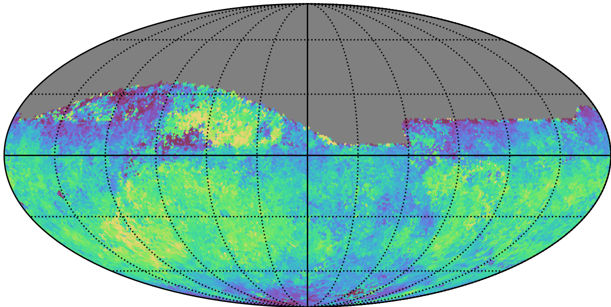
baseline_v3.3_10yrs Yr 1 all bands: Median fiveSigmaDepth
