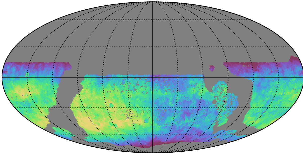
baseline_v3.3_10yrs WFD z band: Median fiveSigmaDepth
