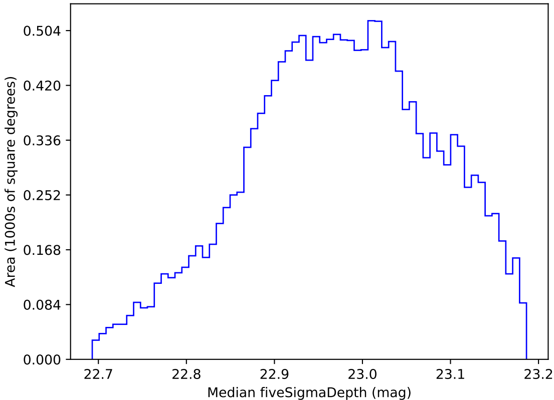
baseline_v3.3_10yrs WFD z band: Median fiveSigmaDepth
