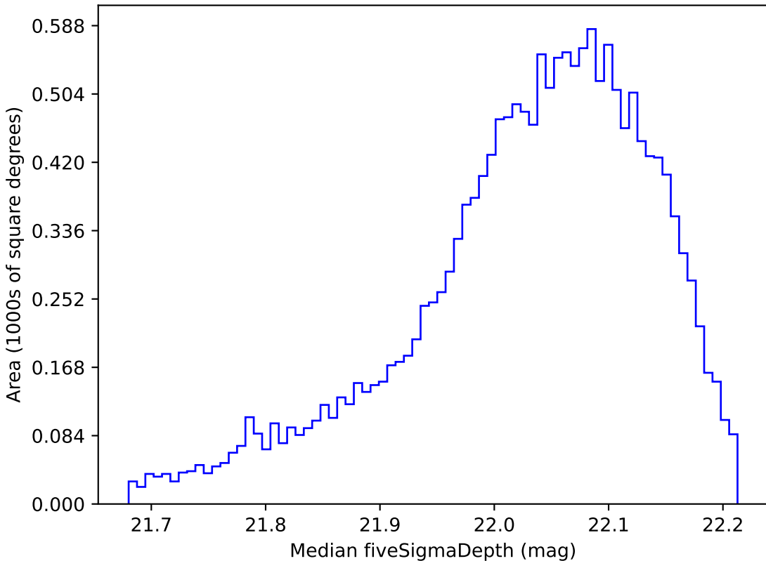
baseline_v3.3_10yrs WFD y band: Median fiveSigmaDepth
