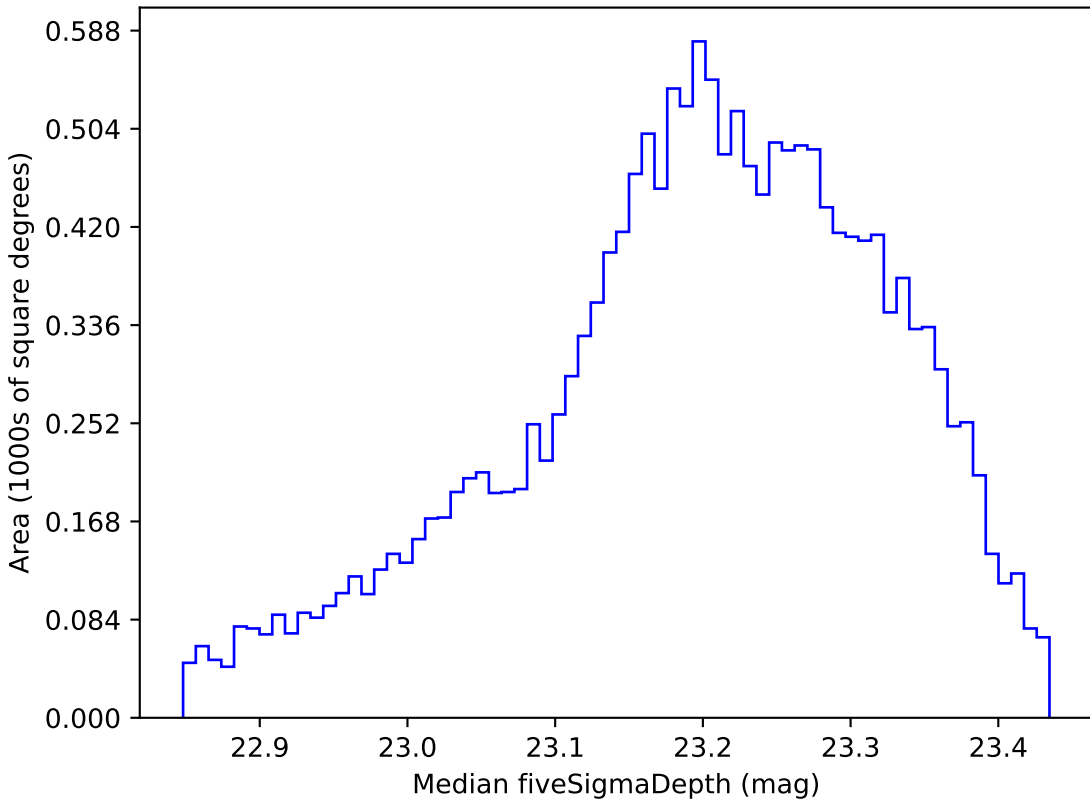
baseline_v3.3_10yrs WFD u band: Median fiveSigmaDepth
