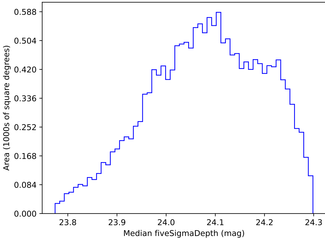
baseline_v3.3_10yrs WFD r band: Median fiveSigmaDepth
