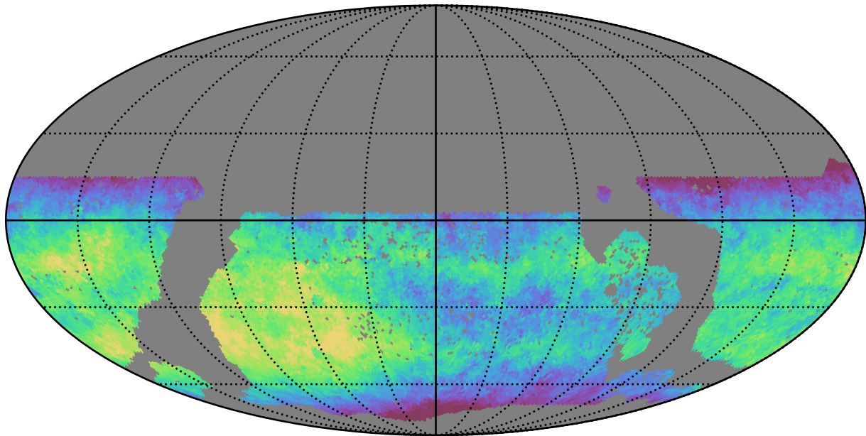
baseline_v3.3_10yrs WFD i band: Median fiveSigmaDepth
