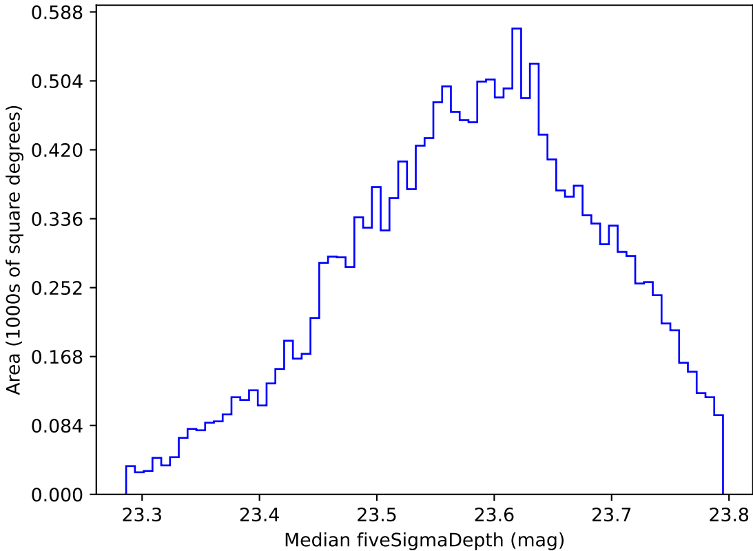
baseline_v3.3_10yrs WFD i band: Median fiveSigmaDepth
