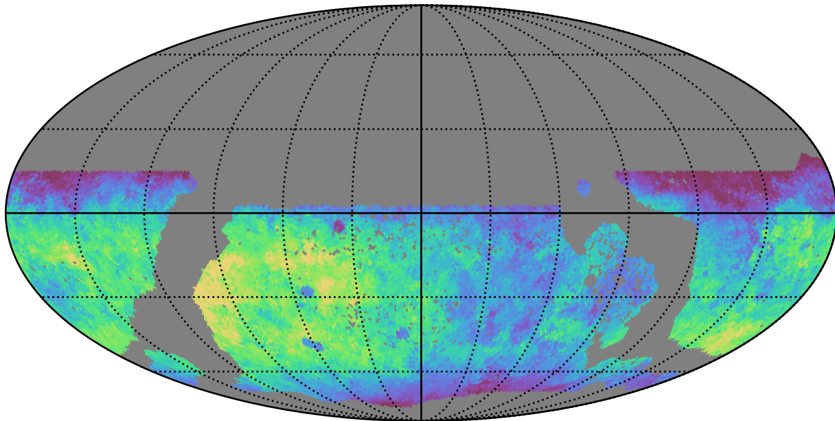
baseline_v3.3_10yrs WFD g band: Median fiveSigmaDepth
