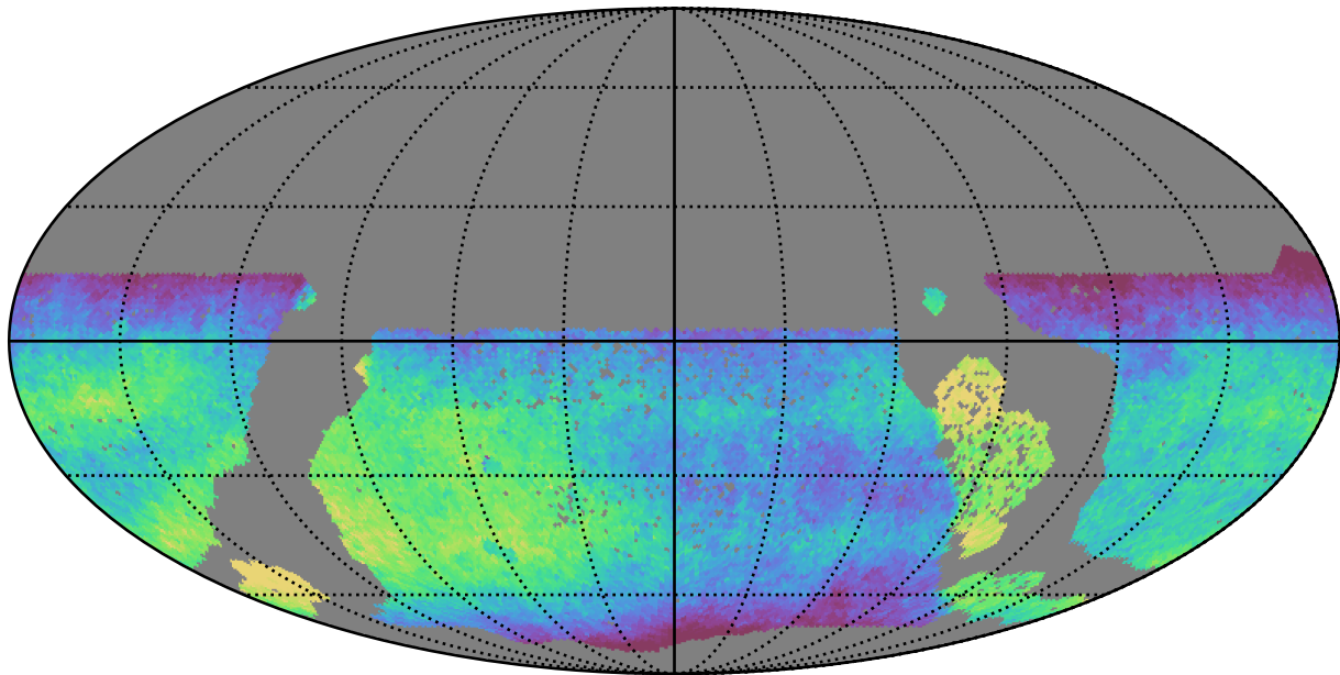
baseline_v3.3_10yrs WFD all bands: Median fiveSigmaDepth
