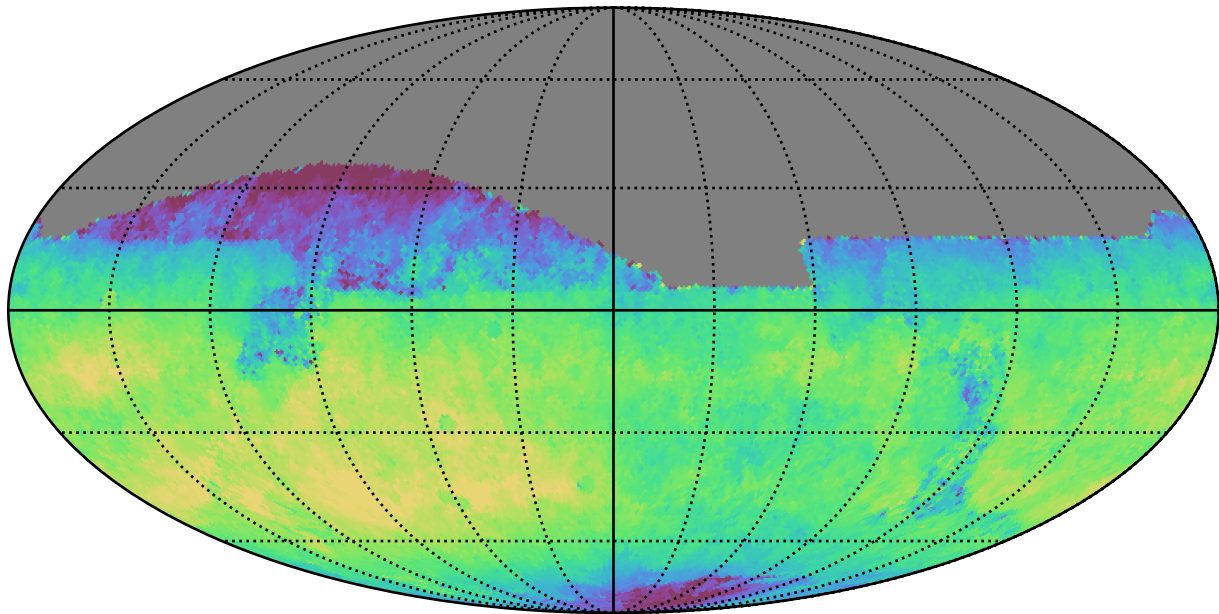
baseline_v3.3_10yrs All sky z band: Median fiveSigmaDepth
