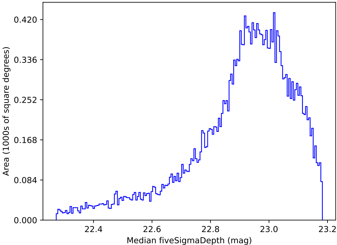
baseline_v3.3_10yrs All sky z band: Median fiveSigmaDepth
