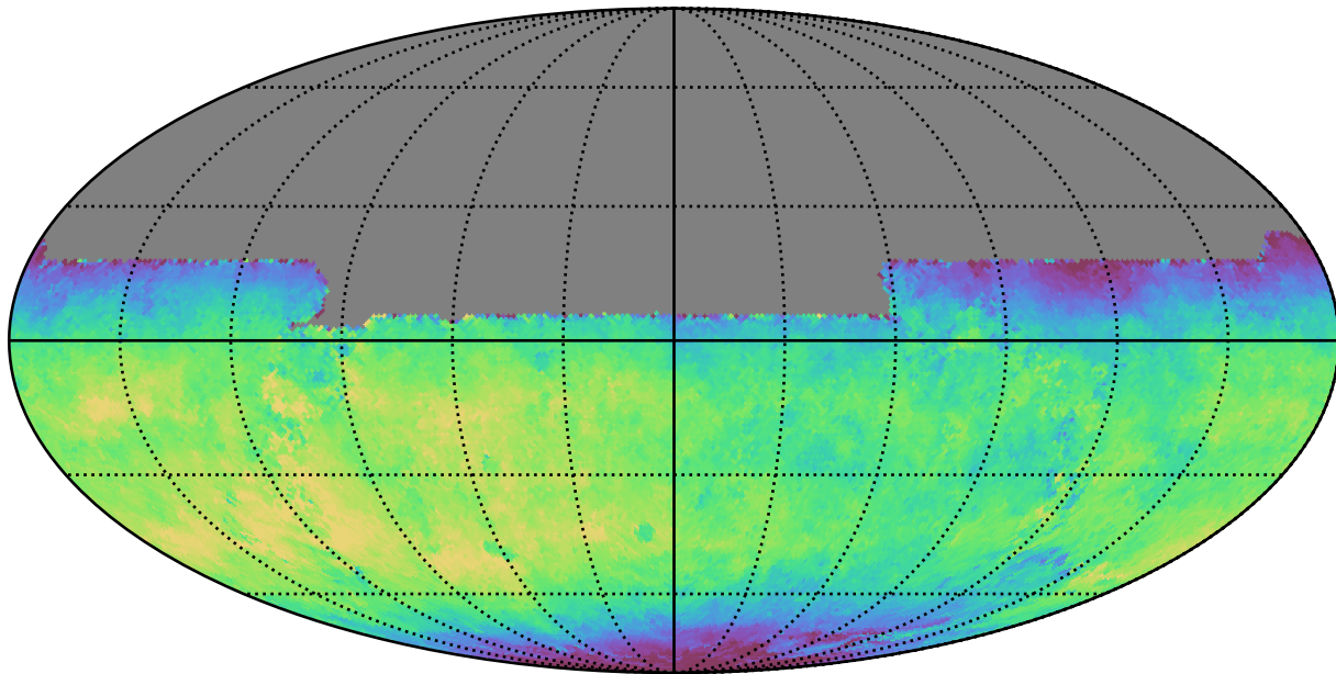
baseline_v3.3_10yrs All sky y band: Median fiveSigmaDepth
