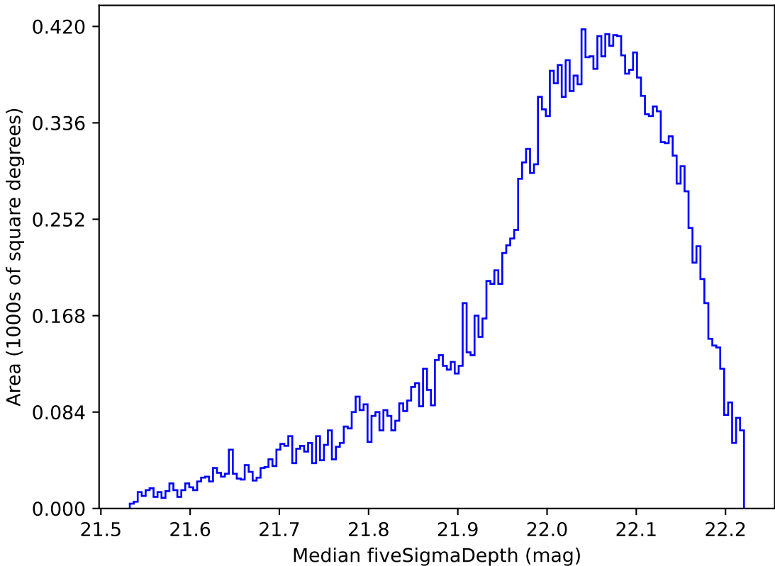
baseline_v3.3_10yrs All sky y band: Median fiveSigmaDepth
