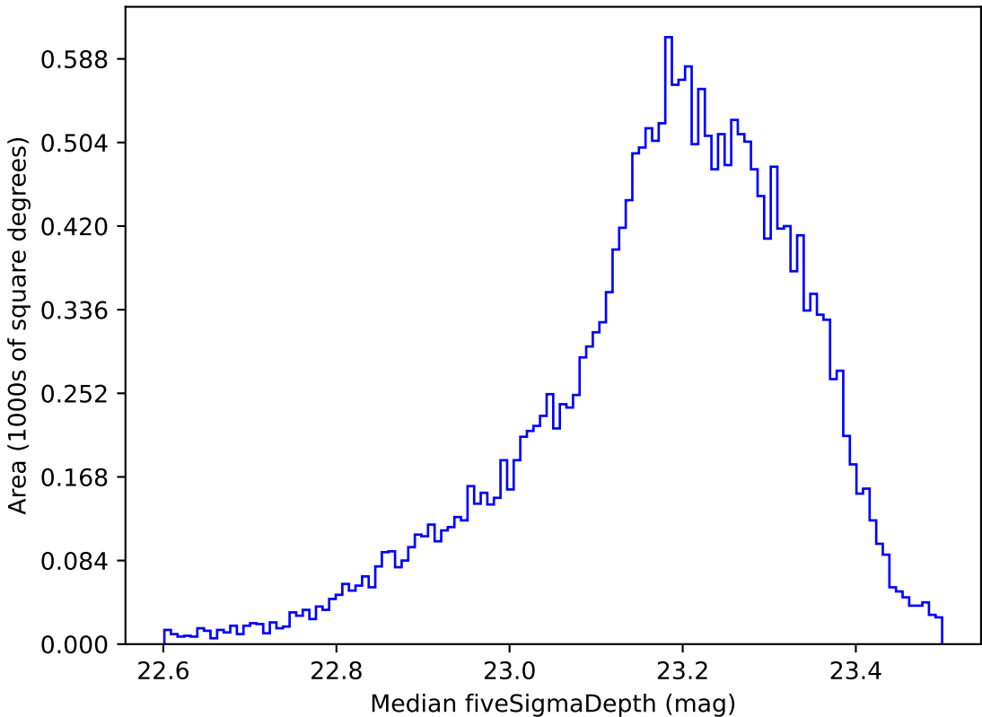
baseline_v3.3_10yrs All sky u band: Median fiveSigmaDepth
