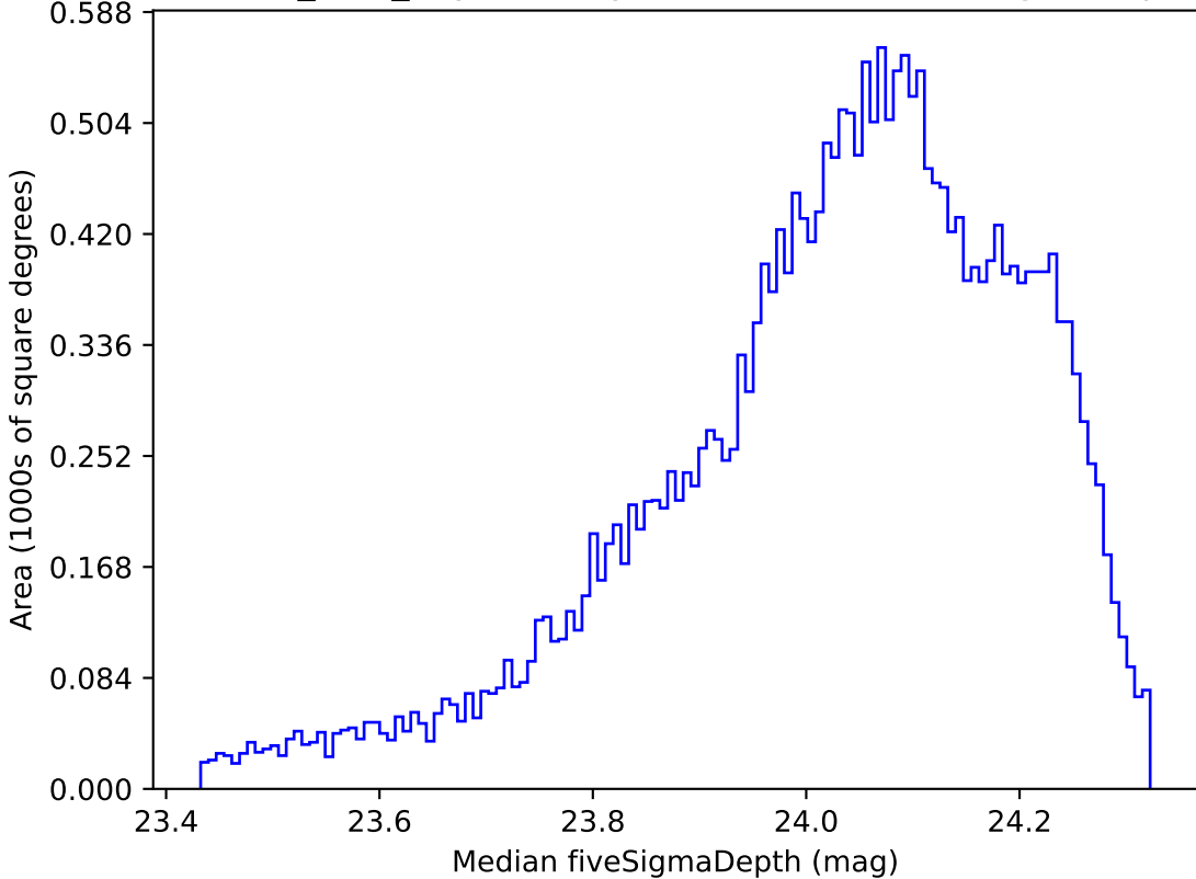
baseline_v3.3_10yrs All sky r band: Median fiveSigmaDepth
