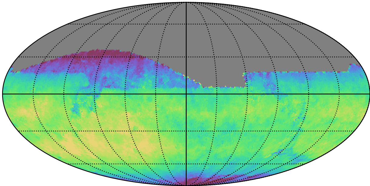
baseline_v3.3_10yrs All sky i band: Median fiveSigmaDepth
