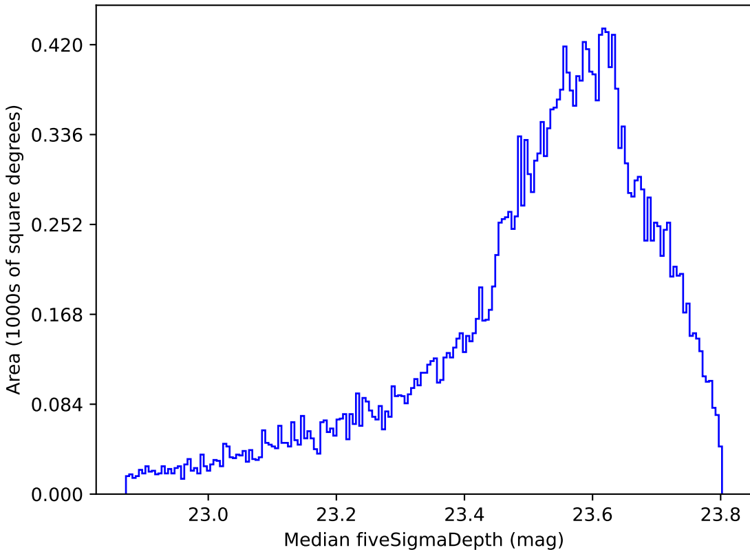
baseline_v3.3_10yrs All sky i band: Median fiveSigmaDepth
