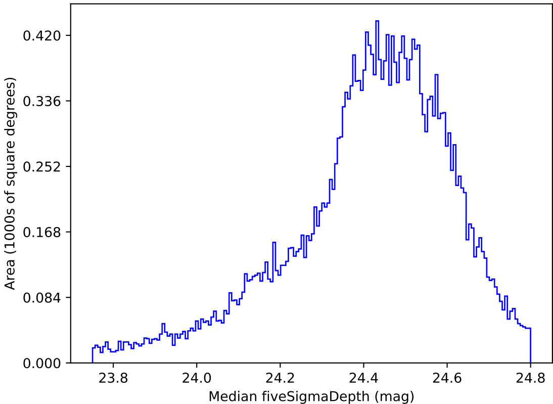
baseline_v3.3_10yrs All sky g band: Median fiveSigmaDepth
