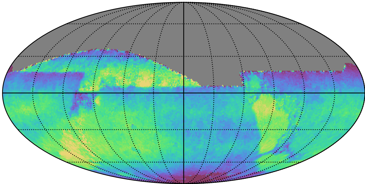
baseline_v3.3_10yrs All sky all bands: Median fiveSigmaDepth
