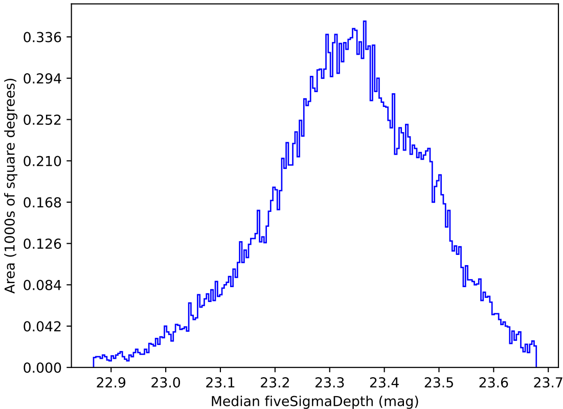
baseline_v3.3_10yrs All sky all bands: Median fiveSigmaDepth
