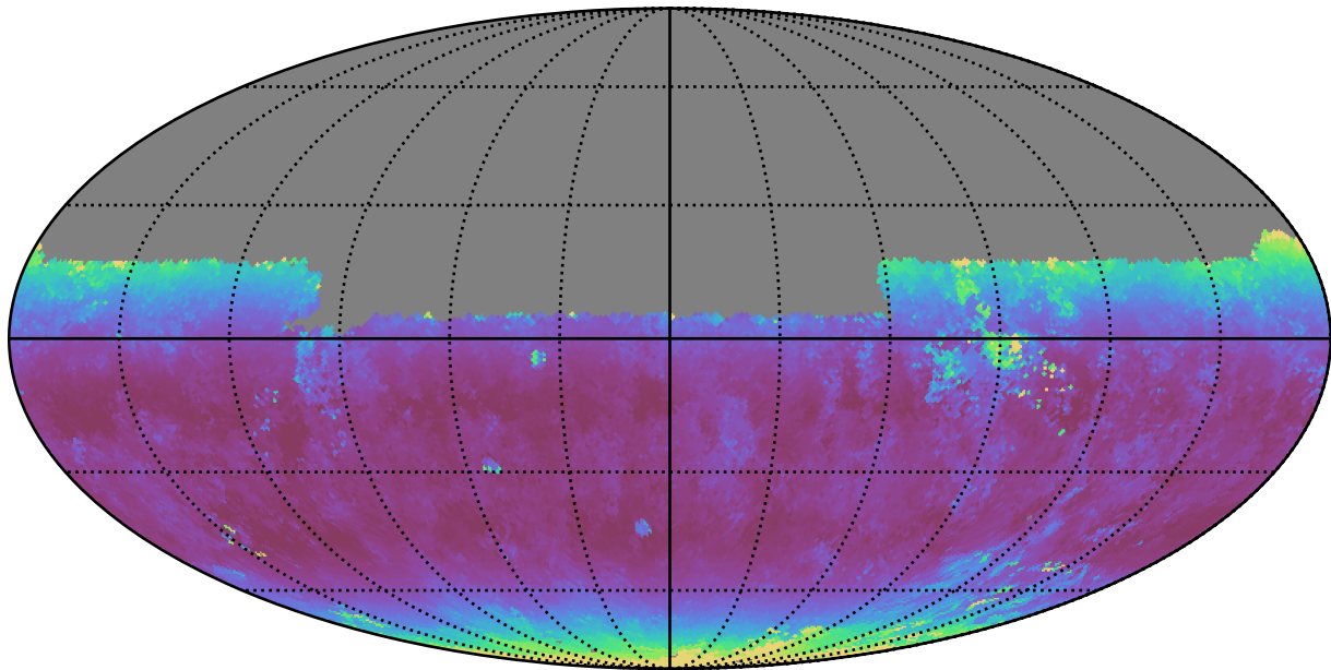
baseline_v3.3_10yrs Yr 1 y band: Median airmass
