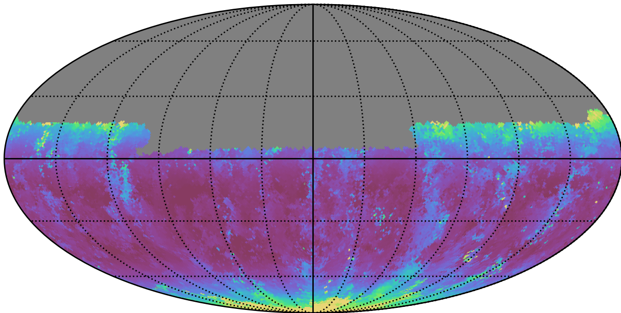
baseline_v3.3_10yrs Yr 1 u band: Median airmass
