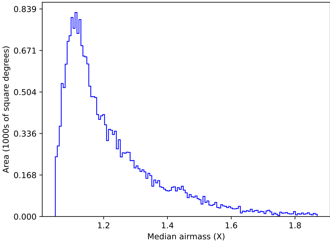
baseline_v3.3_10yrs Yr 1 u band: Median airmass
